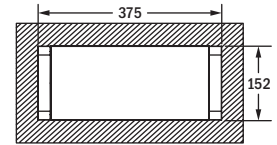
recessed ceiling mounting hollow ceilings
