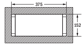
recessed ceiling mounting hollow ceilings
