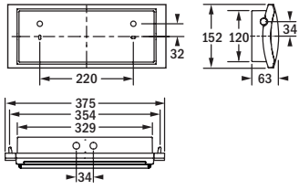
surface wall mounting
