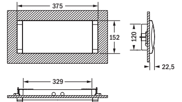
recessed wall mounting hollow walls
