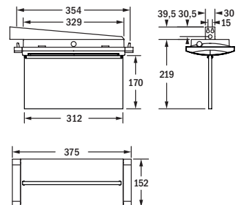
recessed ceiling mounting hollow ceilings
