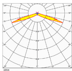
Asymmetric wide-beam
