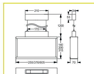
Wire suspension
