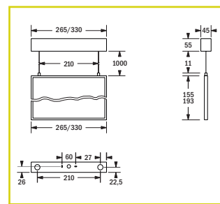
Wire suspension
