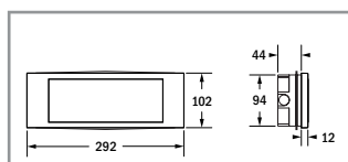
Surface wall and ceiling mounting
