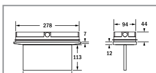
Surface ceiling mounting, display pane
