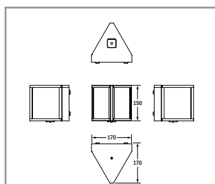
Surface wall mounting (LTO)
