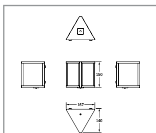
Surface wall mounting (S24 & S230)
