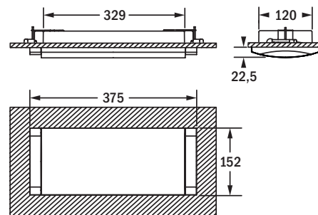
Deckeneinbau (Hohldecke) recessed ceiling mounting (hollow ceiling)
