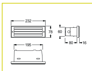
Recessed step mounting (hollow)
