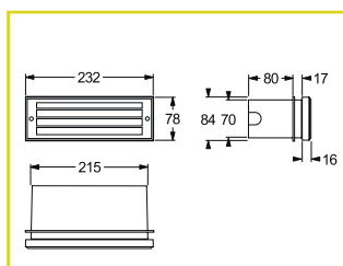
Recessed step mounting (solid)
