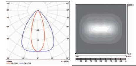
Elliptical optic
