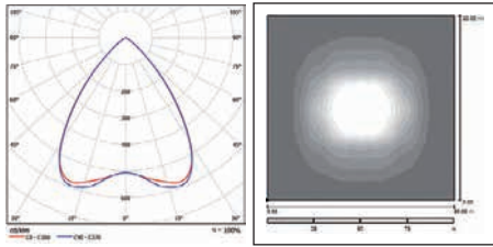
Wide optic
