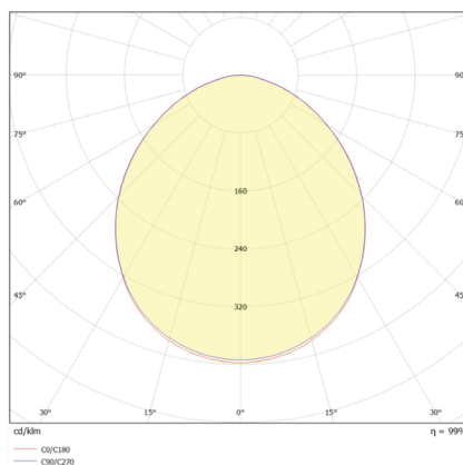
Micro-prism optic system M
