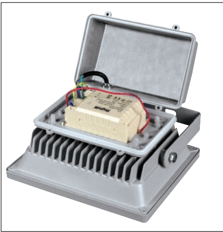
Quick wiring with junction box separated from the light source compartment
