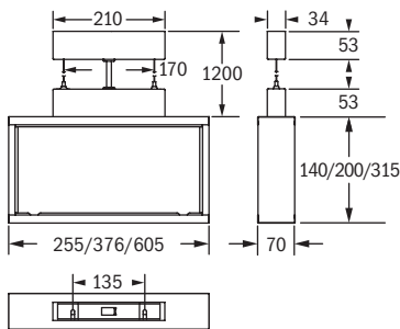
wire suspension
