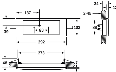
recessed wall mounting (hollow wall)
