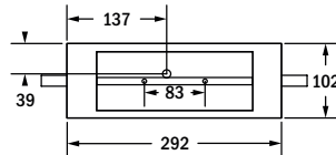
recessed ceiling mounting (hollow ceiling)
