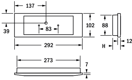
surface wall mounting
