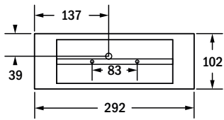
surface ceiling mounting
