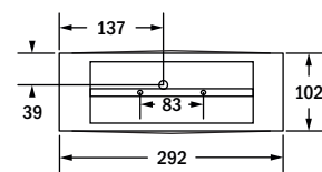
recessed ceiling mounting (solid ceiling)
