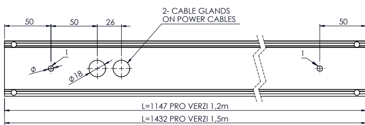
Fig. 4) MOUNTING HOLES
