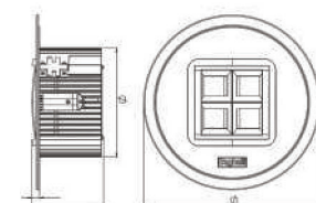
WERSJA DOSTROPOWA Z ADAPTEREM RING / RECESSED VERSION WITH RING ADAPTER
